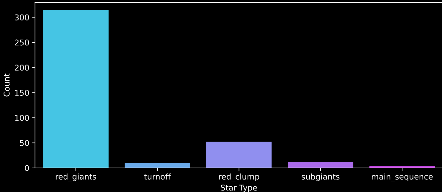
APOGEE DR17 Field: [003-03-C] Count plot of Star Type
