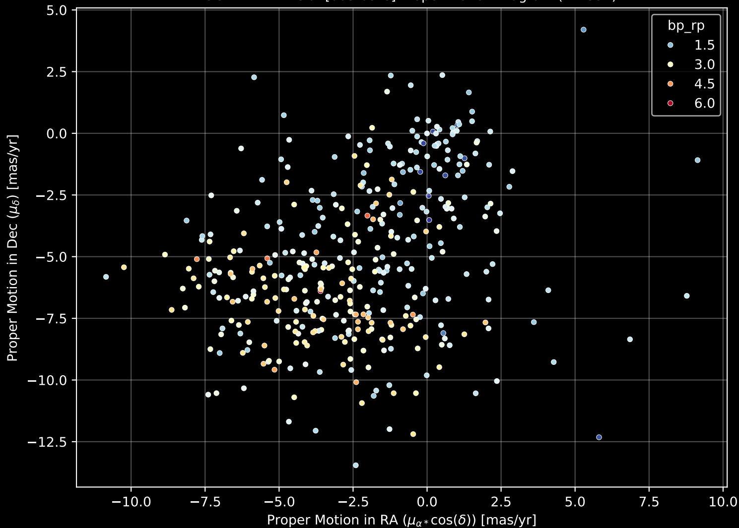
APOGEE DR17 Field: [003-03-C] Proper Motion Diagram (n= 392)
