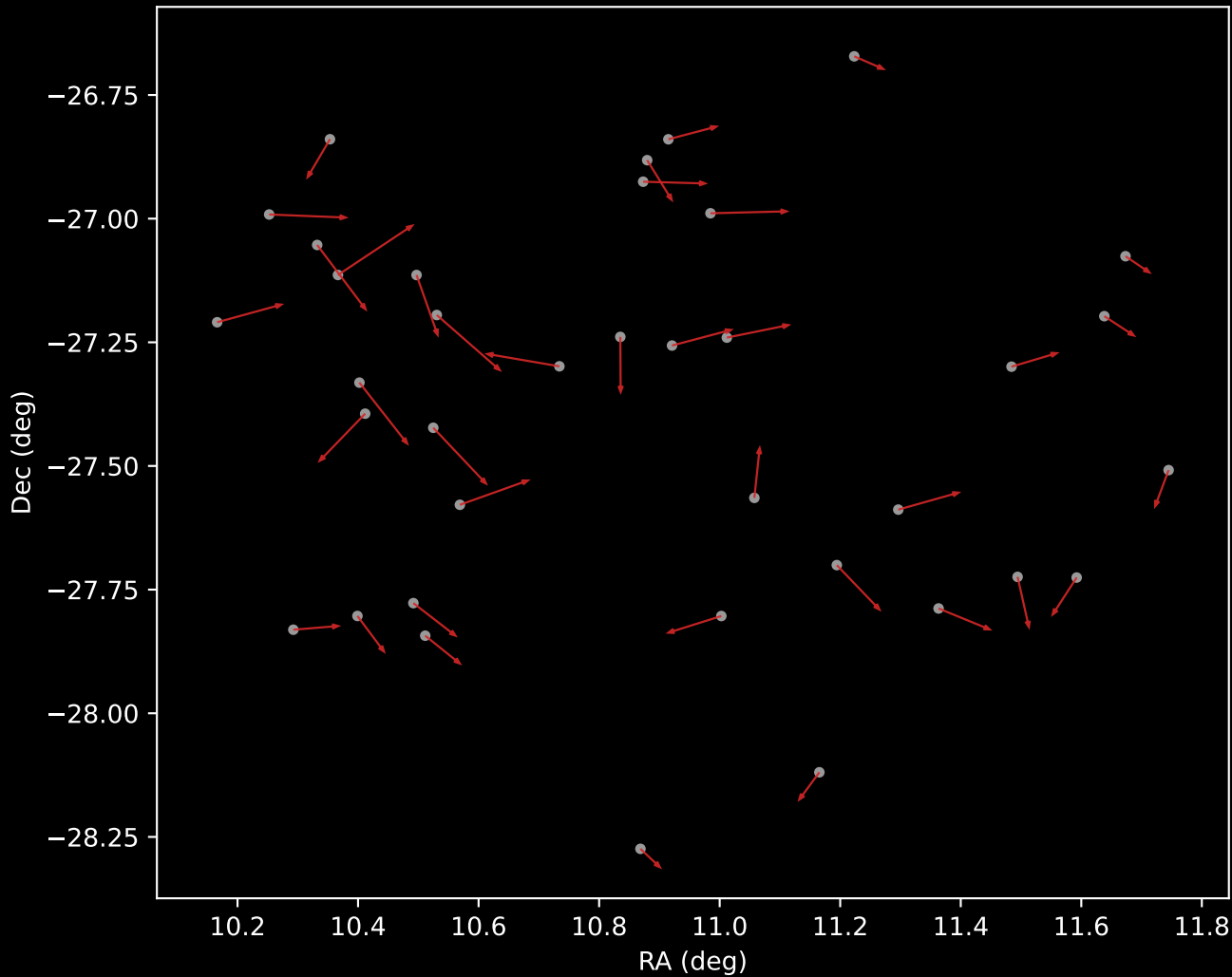
APOGEE DR17 Cluster 6 Proper Motion Vectors (n=37)
