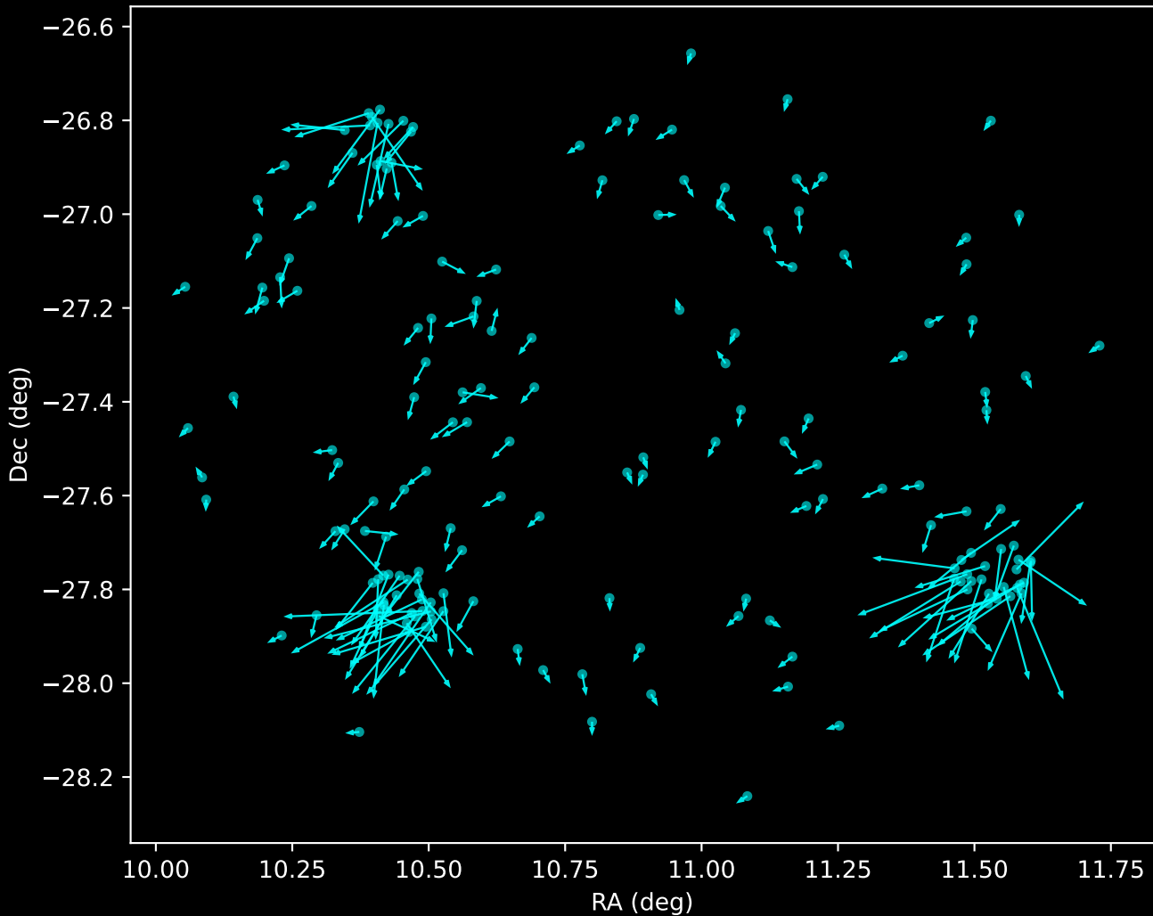
APOGEE DR17 Noise Stream Proper Motion Vectors (n=177)
