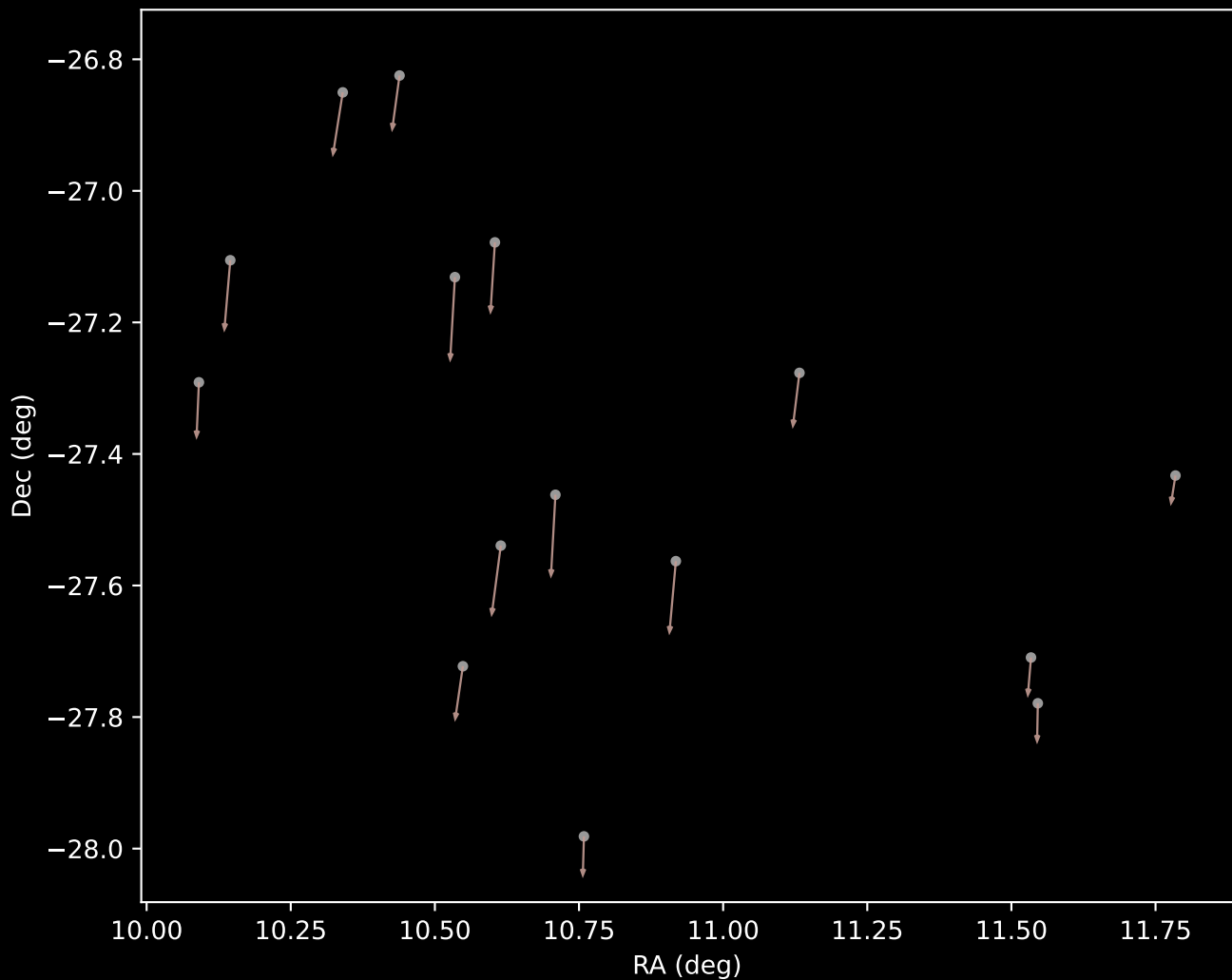
APOGEE DR17 Cluster 11 Proper Motion Vectors (n=15)
