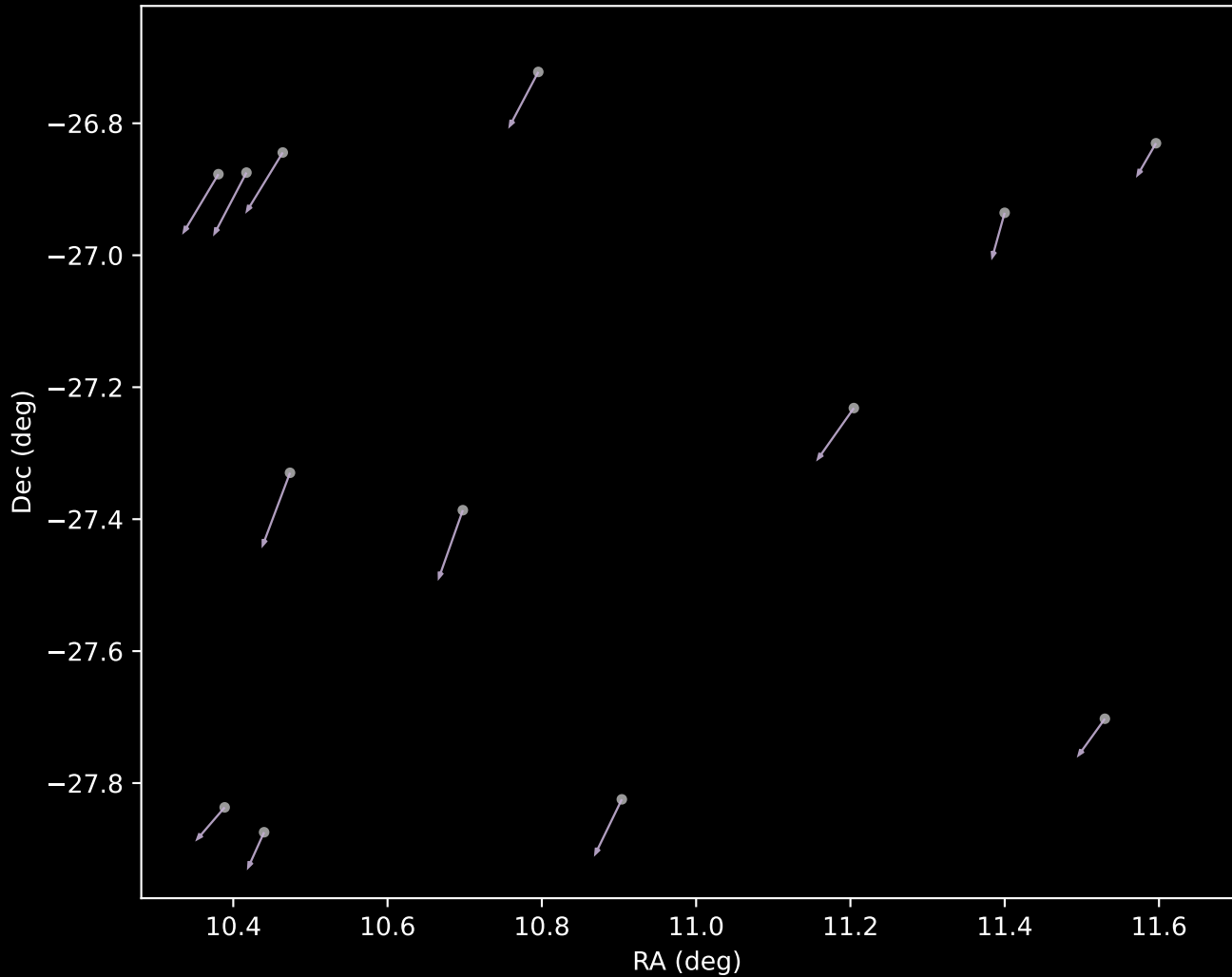
APOGEE DR17 Cluster 9 Proper Motion Vectors (n=13)
