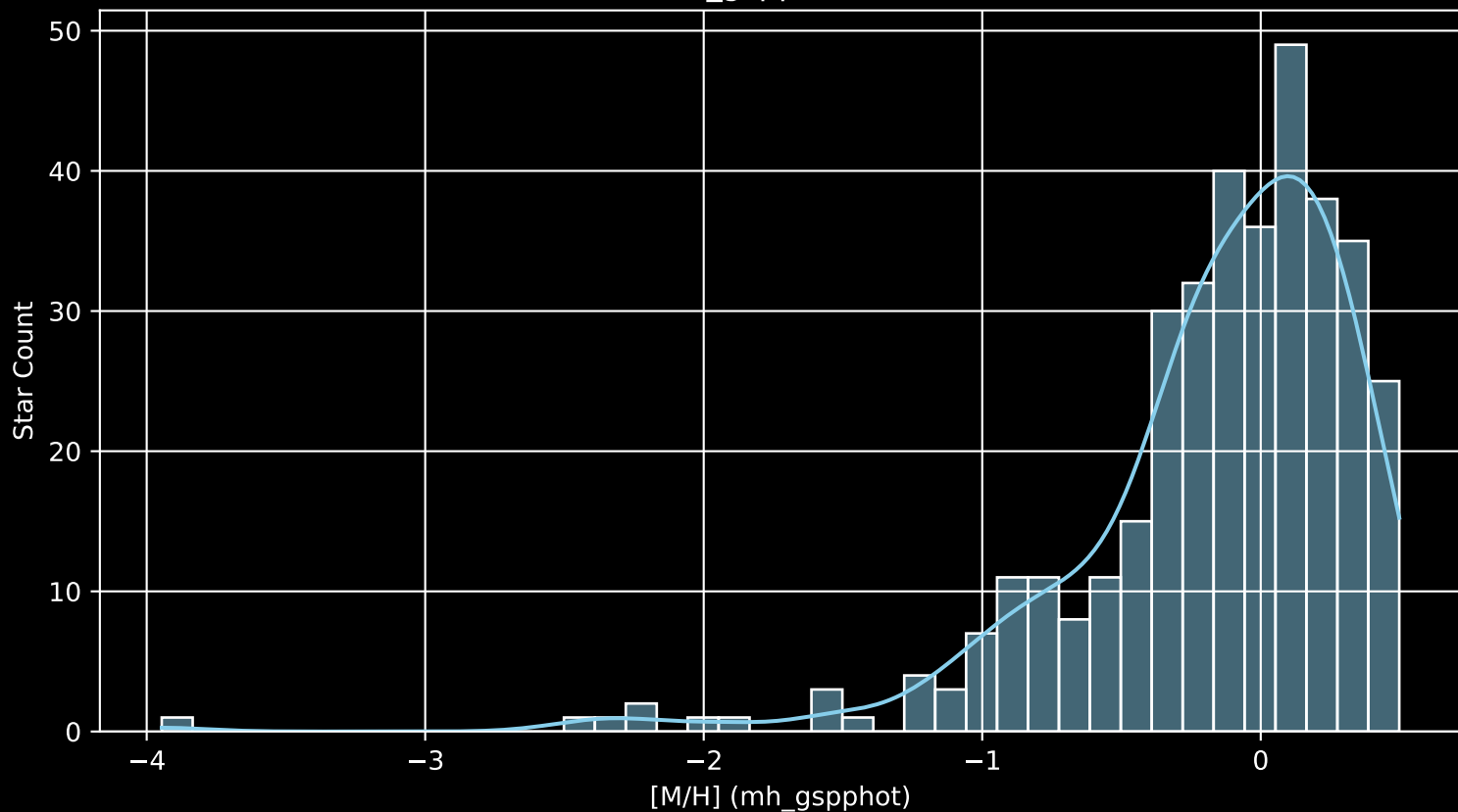
APOGEE DR17 Field: [003-03-C [M/H] (mh_gspphot) (n= 366)
