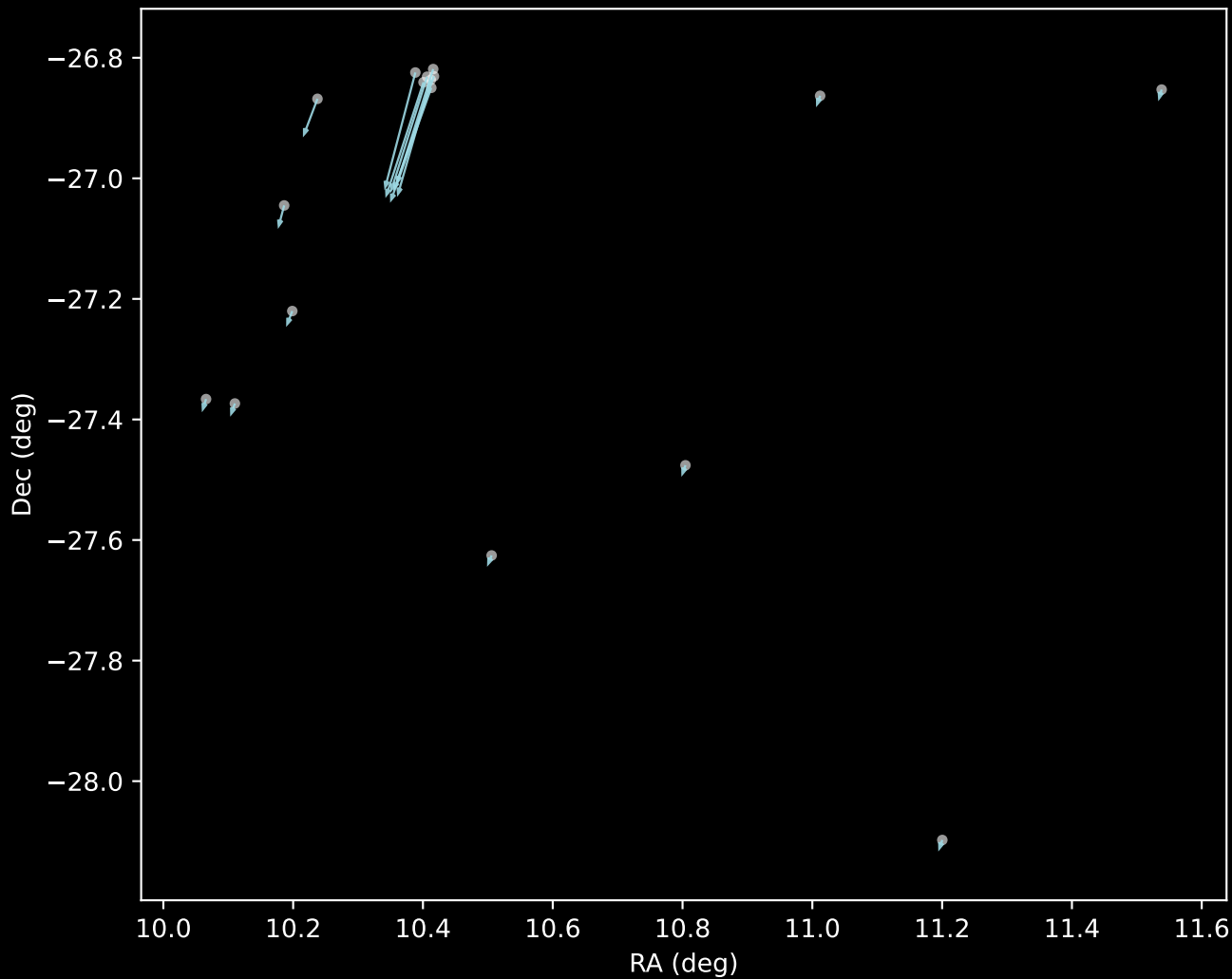
APOGEE DR17 Cluster 19 Proper Motion Vectors (n=17)
