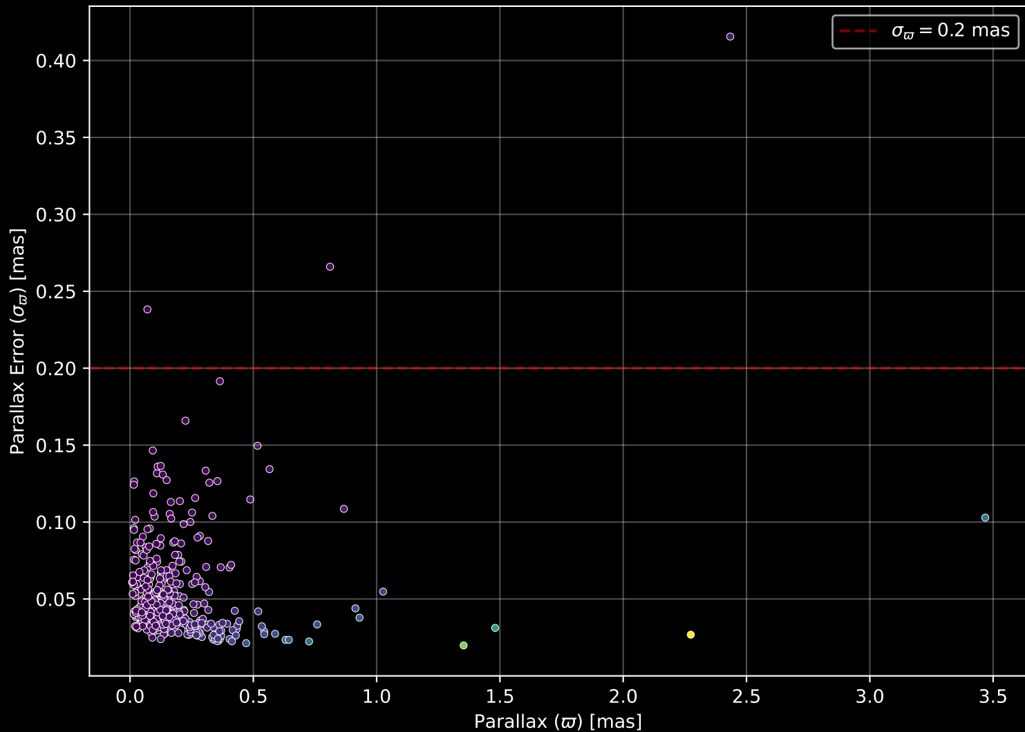
APOGEE DR17 Field: [003-03-C] Parallax Quality (n= 392)
