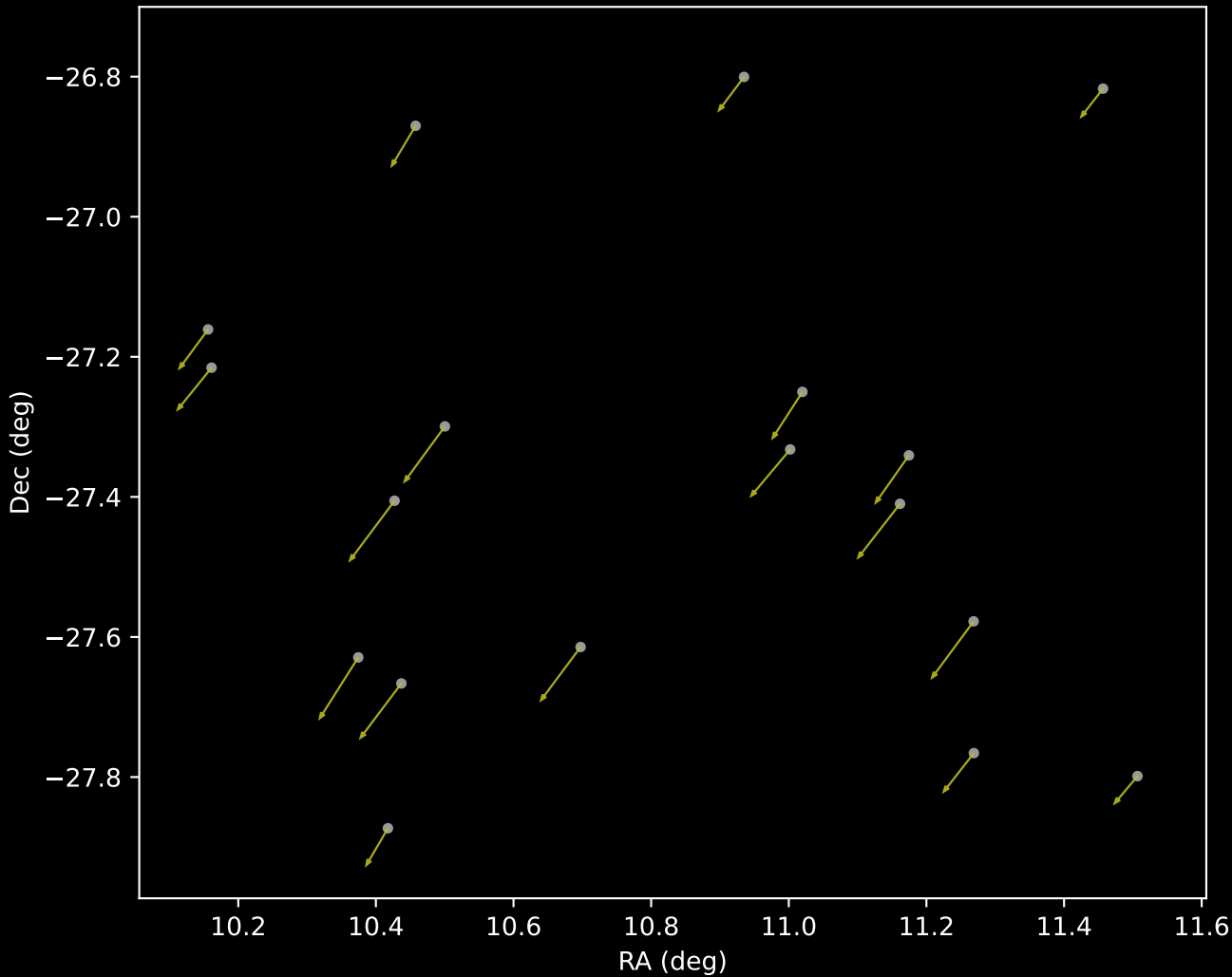
APOGEE DR17 Cluster 16 Proper Motion Vectors (n=18)
