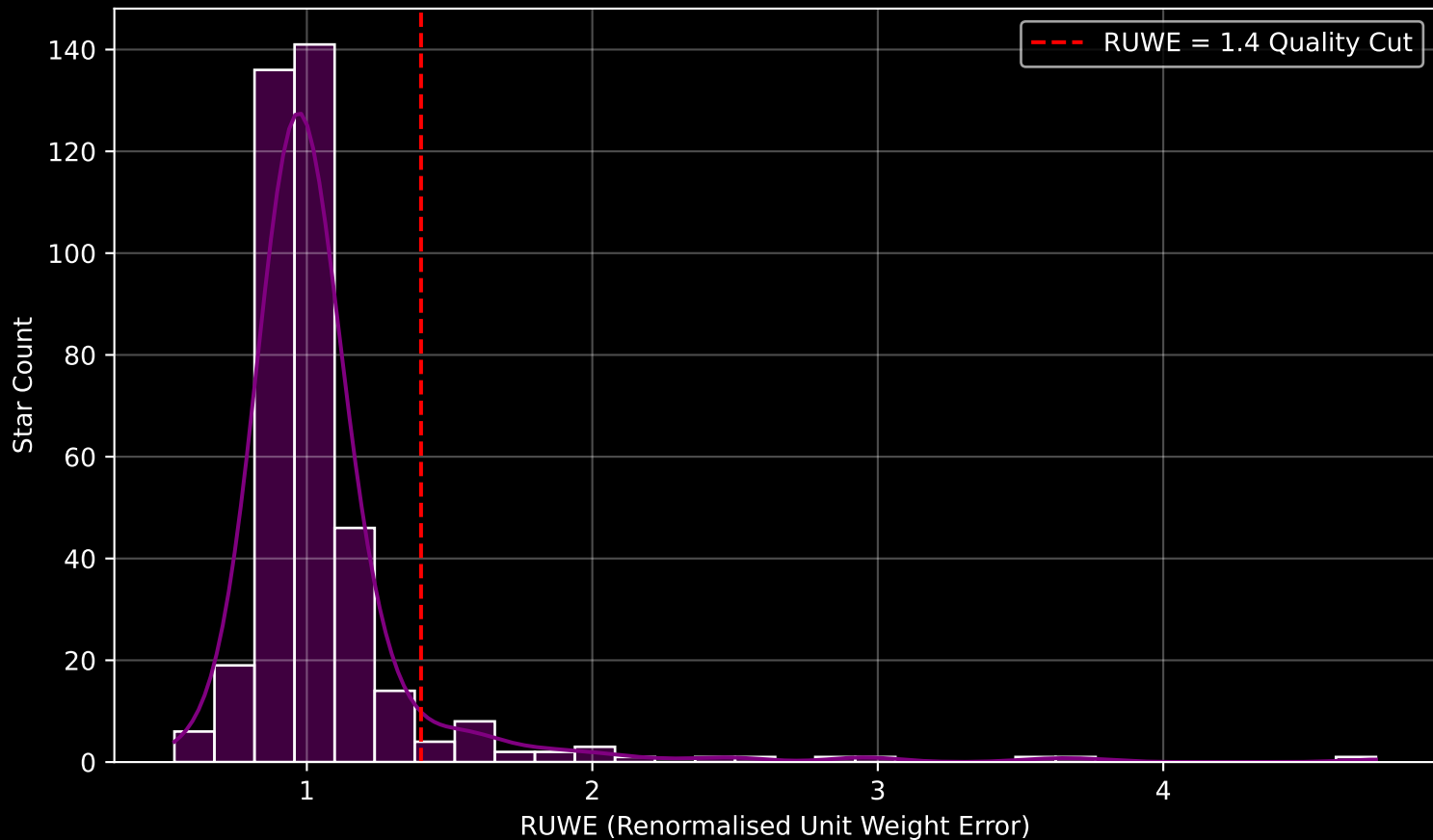
GAPOGEE DR17 Field [003-03-C] RUWE Distribution (n= 389)
